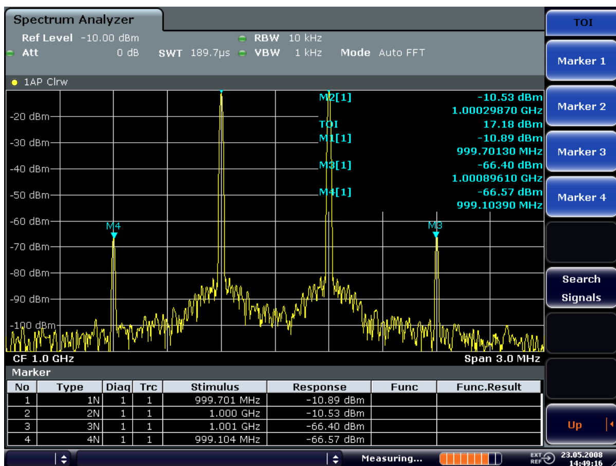
Fig. 5-24: Result of intrinsic intermodulation measurement on the R&S ESRP.
