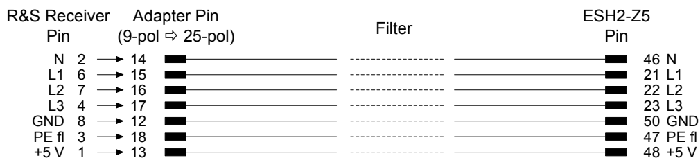
Fig. 4-5: Connection from R&S ESRP to R&S ESH2-Z5
