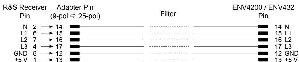
Fig. 4-8: Connection from R&S ESRP to R&S ENV4200 or R&S ENV432
