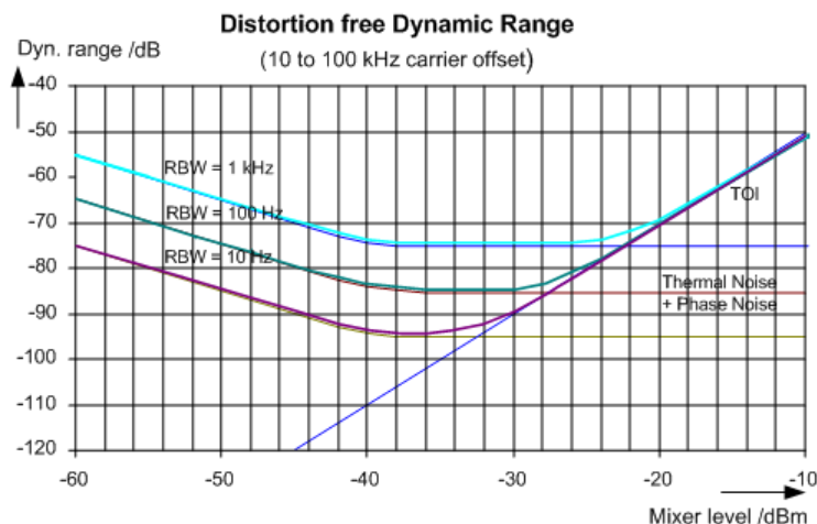
Fig. 5-12: Intermodulation-free dynamic range of the R&S ESRP as a function of level at the input mixer and of the selected resolution bandwidth
