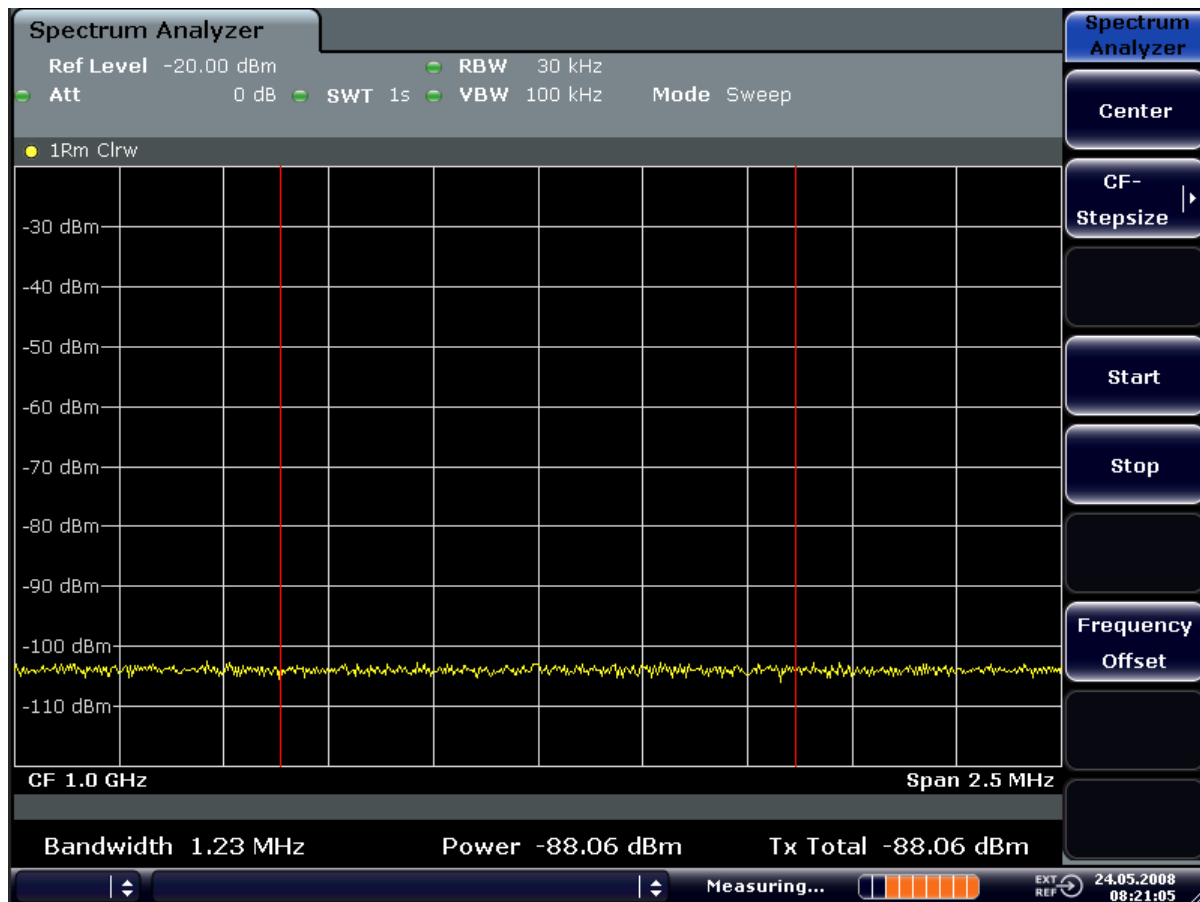
Fig. 5-30: Measurement of the R&S ESRP's intrinsic noise power in a 1.23 MHz channel bandwidth.
