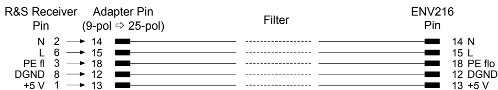
Fig. 4-7: Connection from R&S ESRP to R&S ESH216
