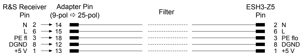
Fig. 4-6: Connection from R&S ESRP to R&S ESH3-Z5
