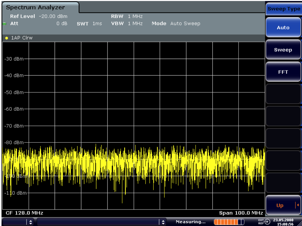
Fig. 5-25: Sine wave signal with low S/N ratio. The signal is measured with the auto peak detector and is completely hidden in the intrinsic noise of the R&S ESRP.
