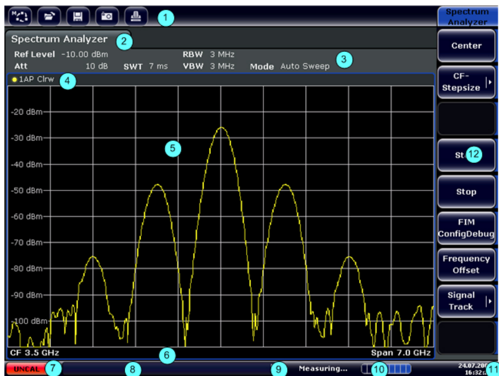
Fig. 2-2: Touchscreen elements
