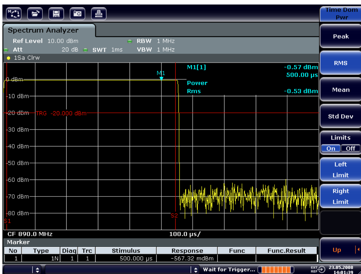
Fig. 2-15: Measurement of the average power during the burst of a GSM signal
