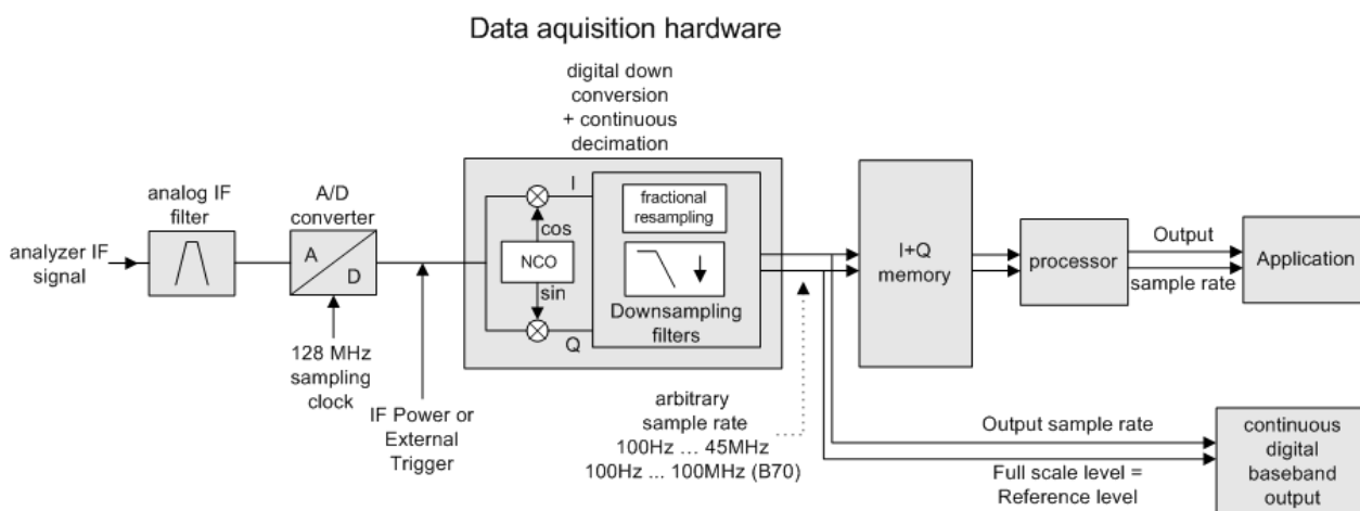
Fig. 6-1: Block diagram illustrating the R&S ESRP signal processing
